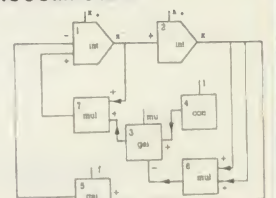
BLOCK DIAGRAM FOR VAN DER POL OSCILLATOR BCSSP Graphics
